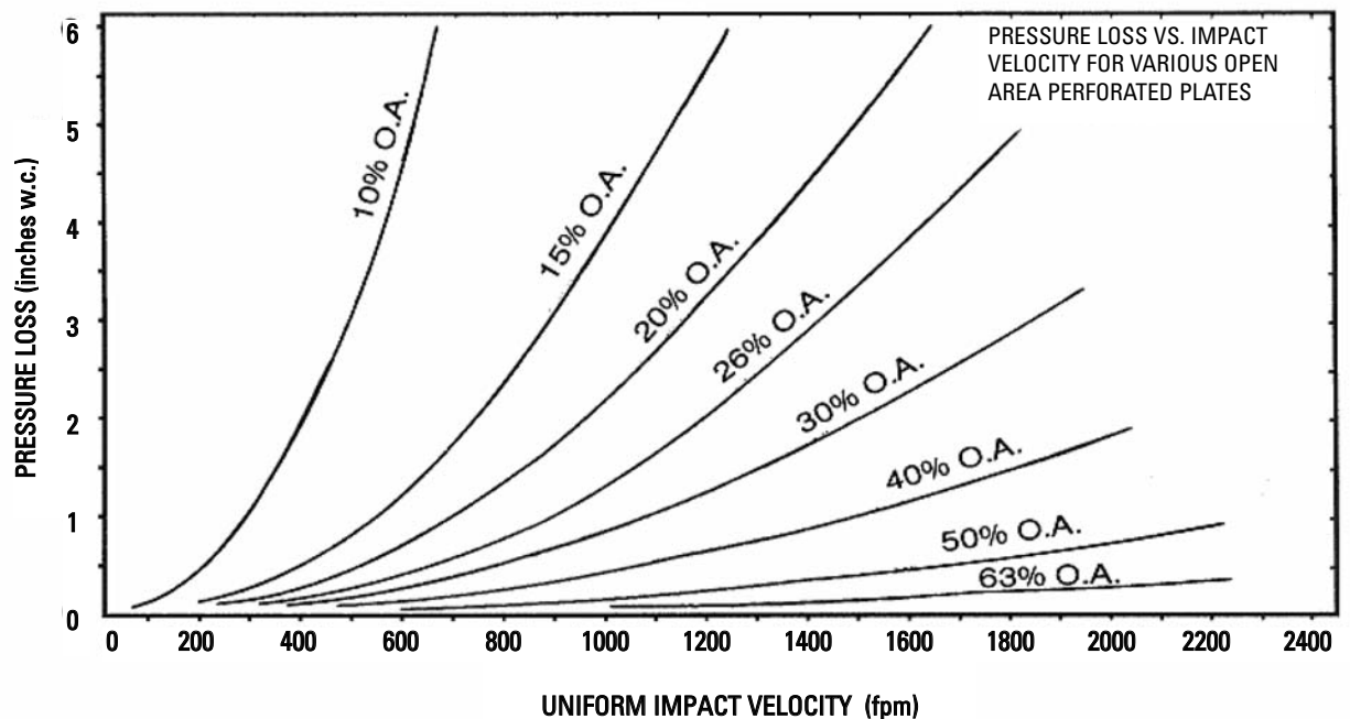
Figure 1, Source: Designers, Specifiers and Buyer's Handbook for Perforated Metals, The Industrial Perforators Association, 1993
