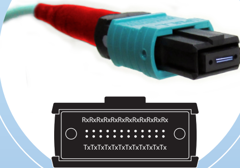
24 Position MPO Assembly
