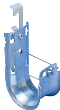
CADDY CAT HP J-Hook to Rod/Wire
