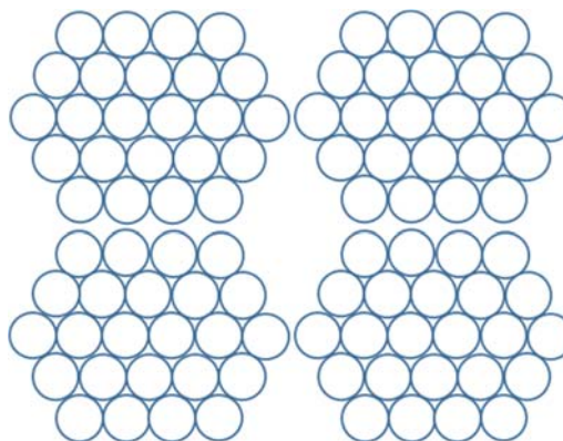
Acceptable deployment of 96 cables using four 24 cable bundles carrying 96 W / 1000 mA over Category 6A 28 AWG
