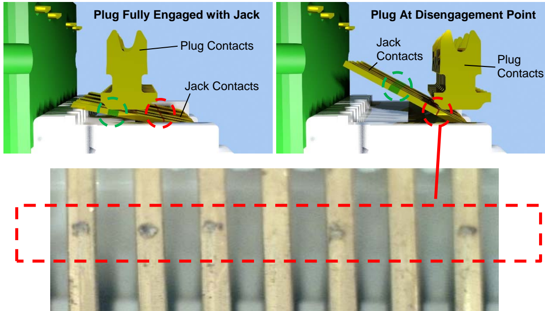
Figure 1: Minor arcing (red) does not occur in Panduit jack mating region (green). Non-Panduit jacks may see such damage in the critical mating area.
