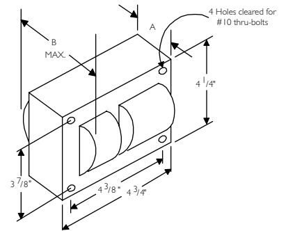
Fig. 2 (4 1/4" x 4 3/4" Core)
