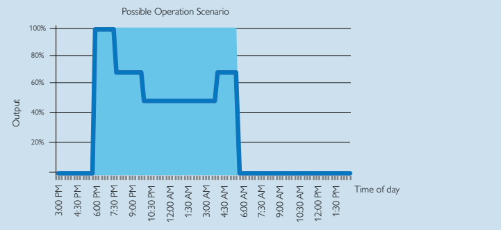
Dynadimmer Standard Programming Schedule
