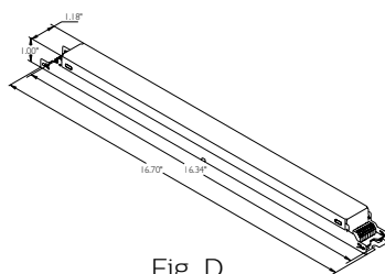
Fig. D Includes connectors with no leads
