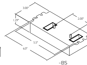
Size 3 Enclosure
