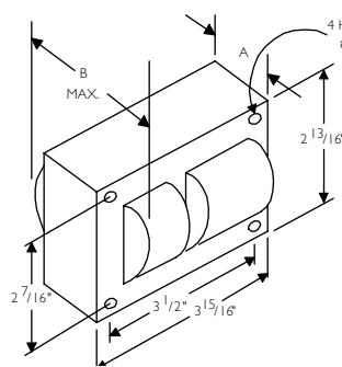
Fig. 1 (3" x 4" Core)
