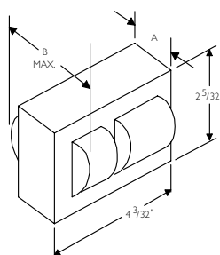
Fig. 6 (2" x 4" Core)
