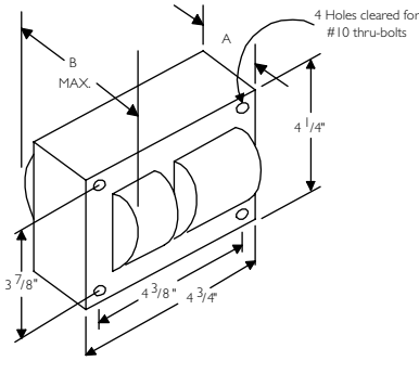
Fig. 2 (4 1/4" x 4 3/4" Core)
