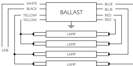
*FOR THREE LAMP OPERATION, INSULATE UNUSED BLUE LEADS INDIVIDUALLY FOR 600V Diag. 66
