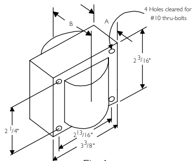
Fig 4 (2 3 / 16 " x 3 3 / 8 " Reactor Core)
