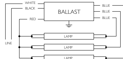
*FOR TWO LAMP OPERATION, INSULATE UNUSED BLUE LEADS INDIVIDUALLY FOR 600V Diag. 65
