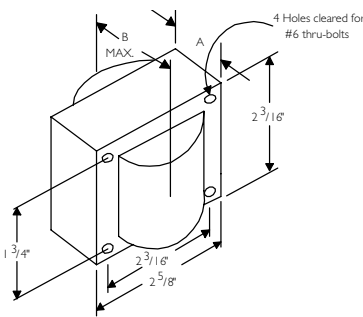
Fig. 9 (2 5 / 8 " x 2 3 / 16 " Reactor Core)
