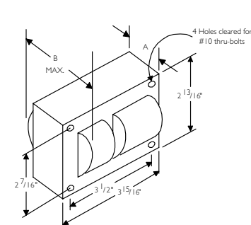
Fig 1 (3" x 4" Core)
