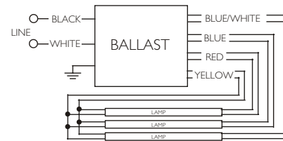
*INSULATE UNUSED LEADS INDIVIDUALLY FOR 600V Diag. 178
