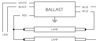
*FOR SINGLE LAMP OPERATION, INSULATE UNUSED BLUE LEAD FOR 600V Diag. 64
