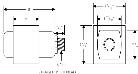
Fig 11 (J-Box Ballast)
