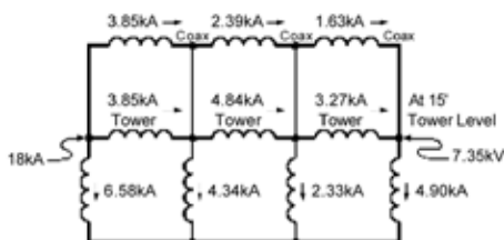
Average Proportional Coax Current is 2.733kA.
