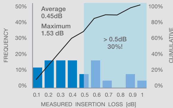
Figure 4. Insertion loss splice test result with poor cleaves (Normally the caution window appears on the screen so the splices are intentional operation.)
