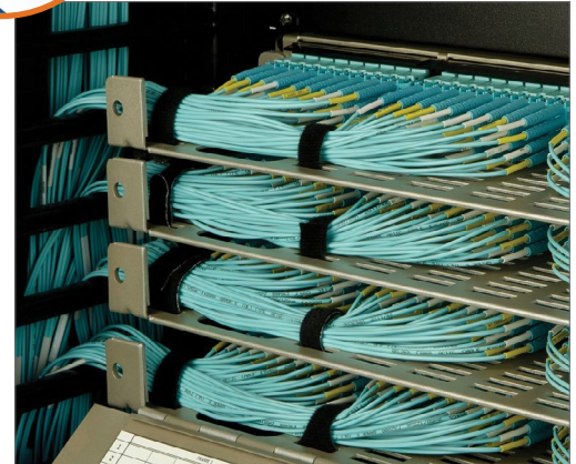
Up to 72 LC Duplex ports per 1RU of space
