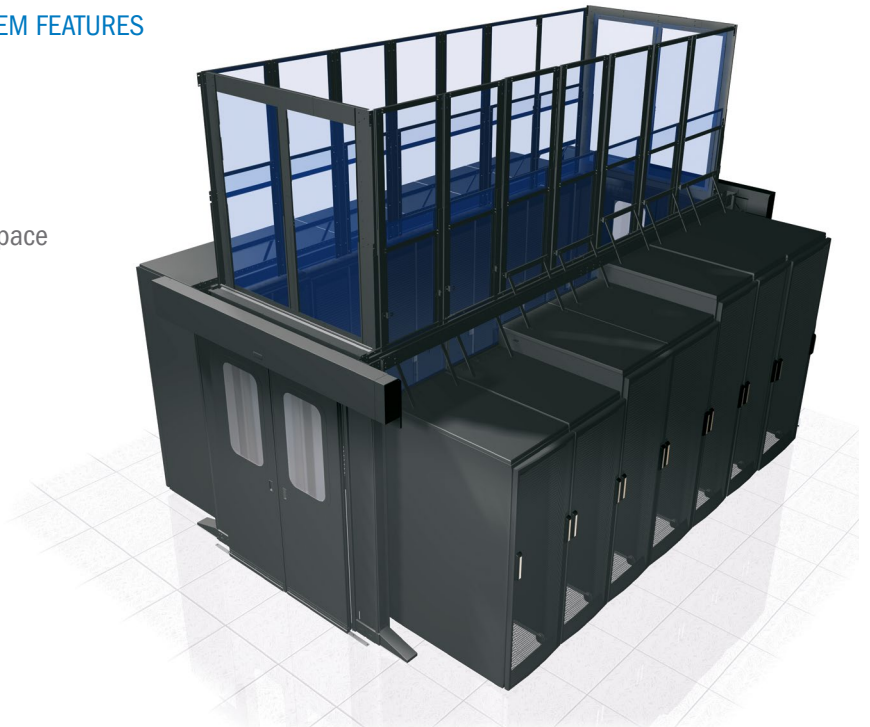
Vertical wall containment typically used for hot aisle or ceiling discharge cold aisle containment
