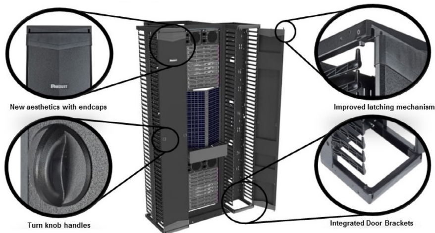
PatchRunner 2 highlights
