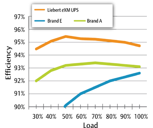
Liebert eXM UPS (40 kVA/kW, 208 V) in double-conversion mode
