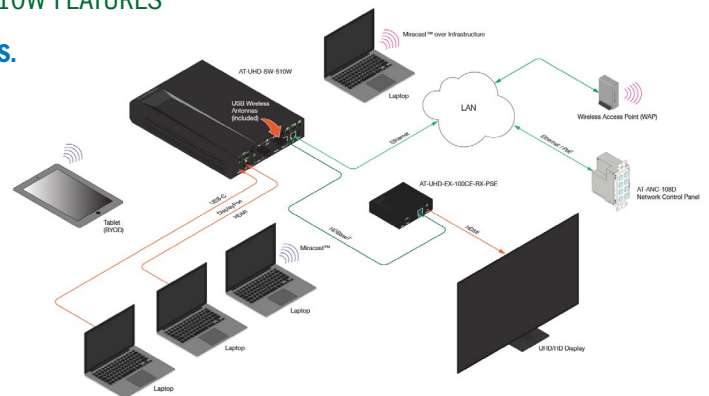
Wired and Wireless A/V Presentation System for BYOD
