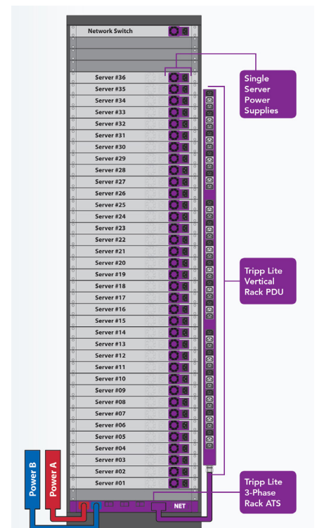
Patent pending three-phase rack ATS provides redundant power to each server's power supply individually.
